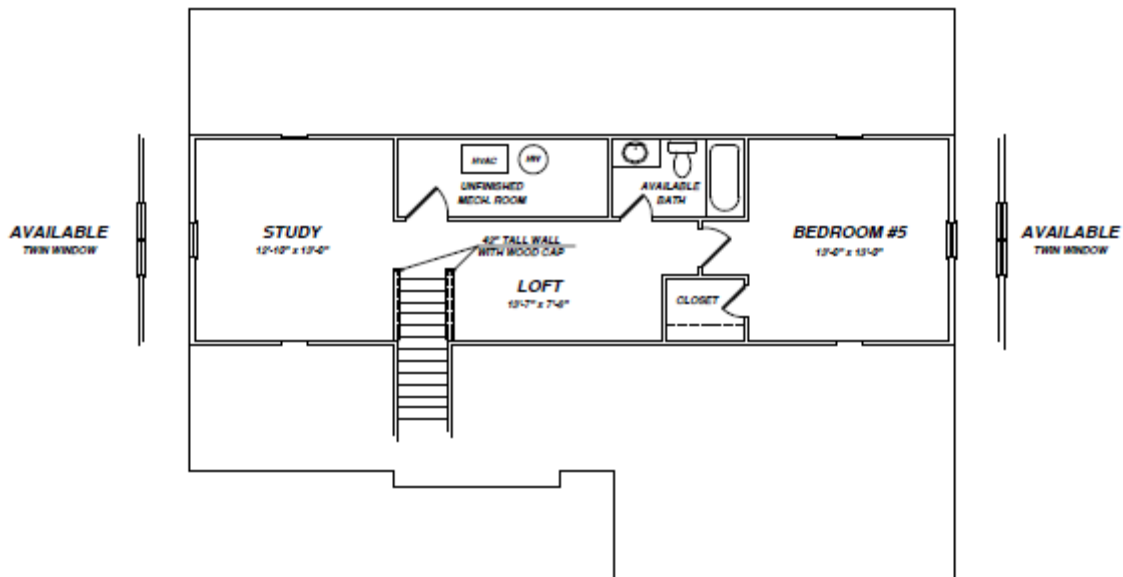
AVAILABLE THIRD FLOOR PLAN W/ OPTIONAL LAYOUT #2 W/O ADDED CLOSET
