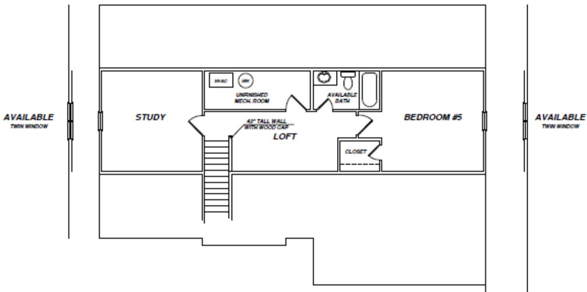
AVAILABLE THIRD FLOOR PLAN W/ OPTIONAL LAYOUT #2
