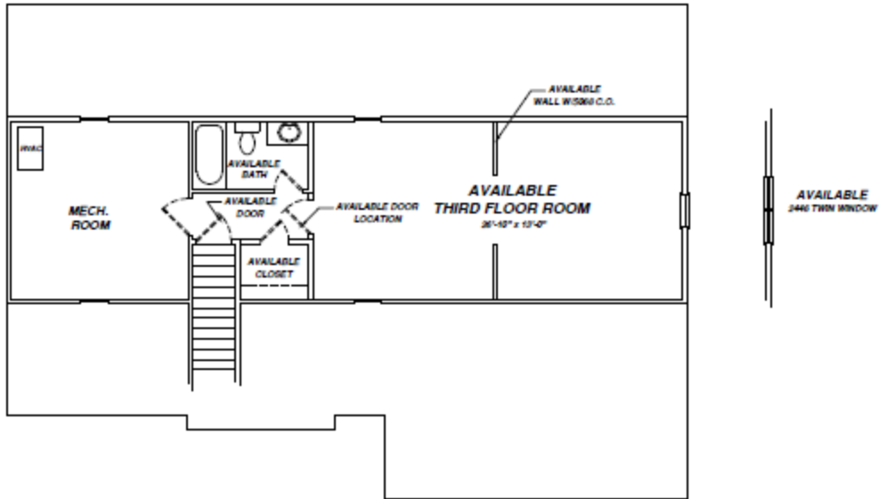
AVAILABLE THIRD FLOOR PLAN W/ OPTIONAL LAYOUT #1
